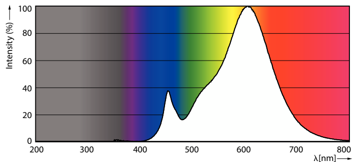
Spectral Power Distribution Colour - MAS LEDcandle DT 5.5-40W B22 B38 CL UK
