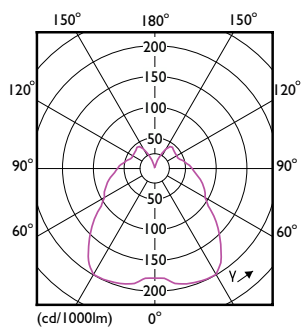
Light Distribution Diagram - MAS LEDcandle DT 5.5-40W B22 B38 CL UK
